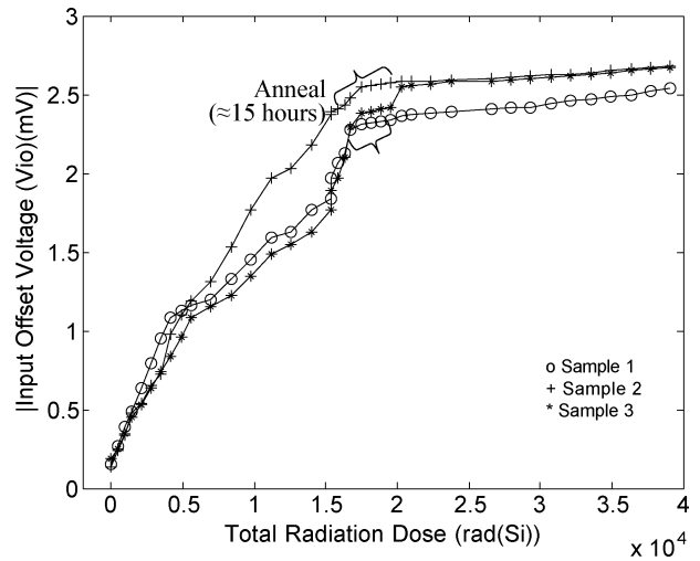
Fig. 7. Variation of V_{io} of AD549JH, as a function of total irradiation dose.
