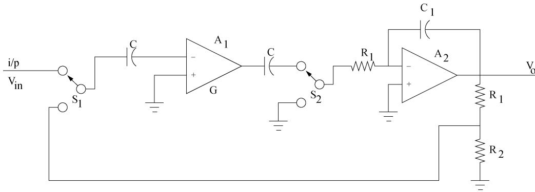
Fig. 13. Internal circuit diagram of a chopper-stabilized configuration in an op-amp.
