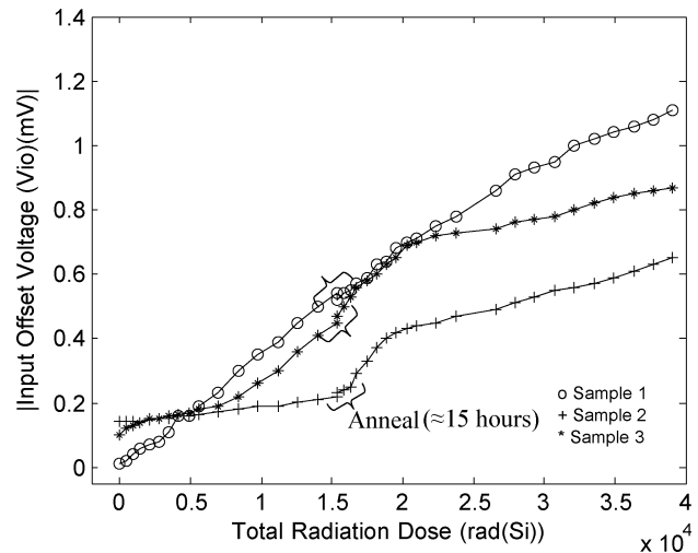
Fig. 9. Variation of V_{io} of OPA128JM, as a function of total irradiation dose.
