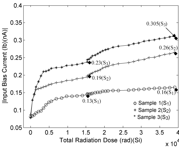
Fig. 15. Variation of I_b of TC7652, as a function of total irradiation dose.
