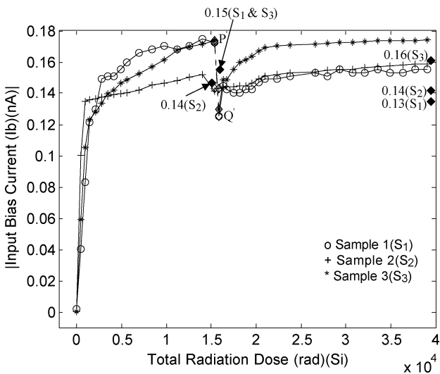
Fig. 6. Variation of I_b of DN8500A, as a function of total irradiation dose.
