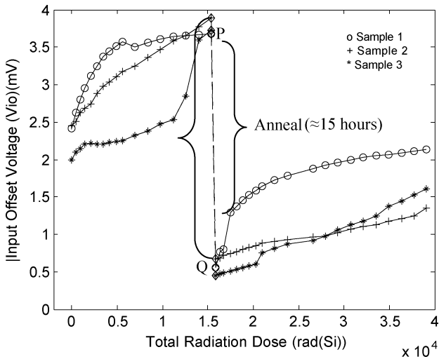
Fig. 5. Variation of V_{io} of DN8500A, as a function of total irradiation dose.
