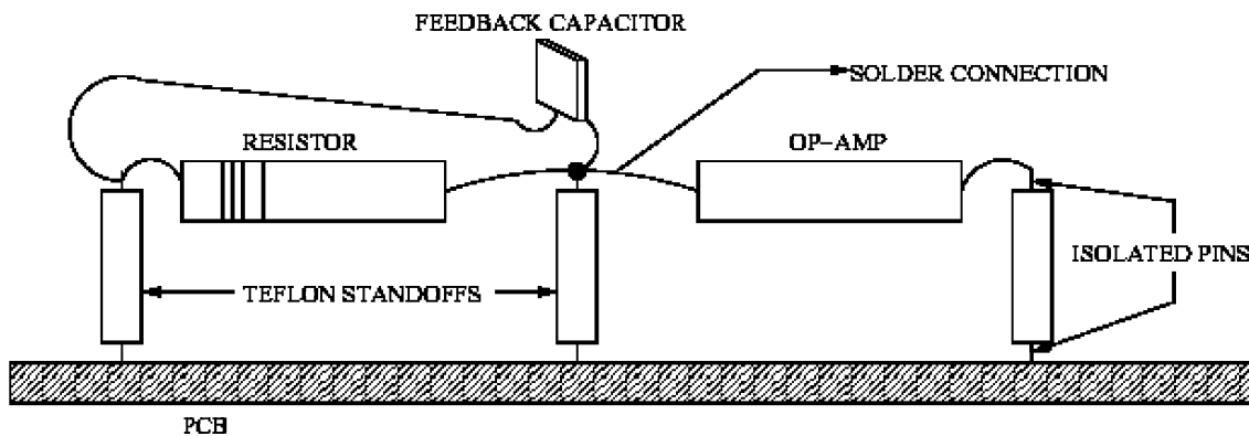
Fig. 4. Quality PCB design for ULIBC linear devices using Teflon standoffs, where air-wiring is used (input pins of the ULIBC op-amp are lifted out of the PCB and soldered onto the Teflon standoffs, so that there is an inherent isolation between the pins and the PCB).
