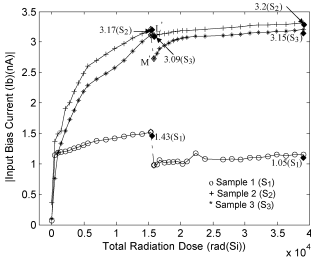
Fig. 10. Variation of I_b of OPA128JM, as a function of total irradiation dose.
