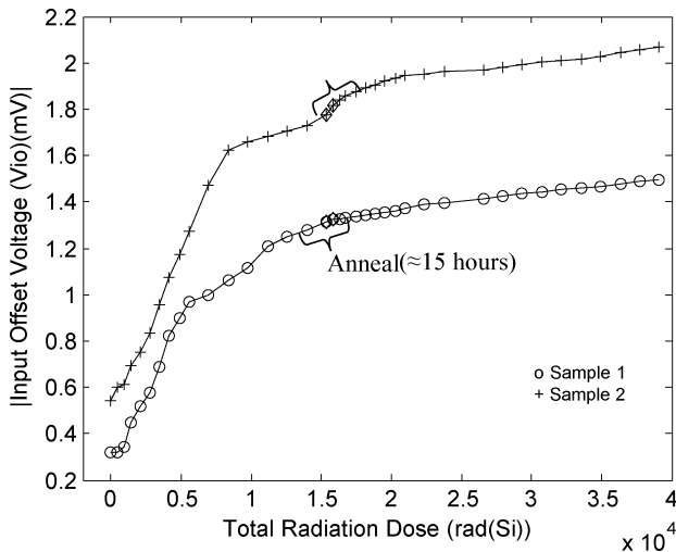
Fig. 11. Variation of V_{io} of LMC6001AIN, as a function of total irradiation dose.
