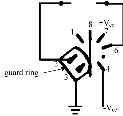
Fig. 3. PCB layout of the scheme used in measurement of nascent characteristics of ULIBC linear devices having TO-99 metal can package.
