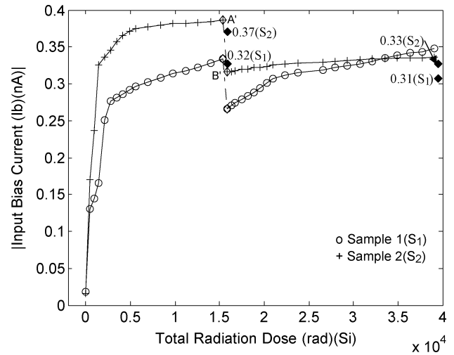
Fig. 12. Variation of I_b of LMC6001AIN, as a function of total irradiation dose.
