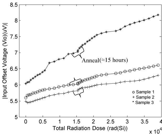
Fig. 14. Variation of V_{io} of TC7652, as a function of total irradiation dose.
