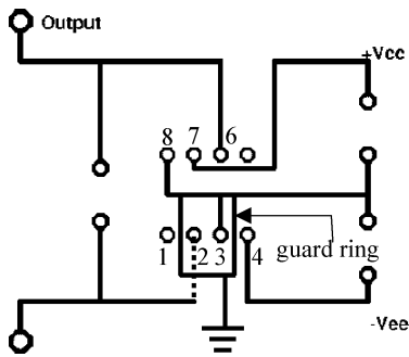
Fig. 2. PCB layout of the scheme used in measurement of nascent characteristics of ULIBC linear devices having DIP plastic package.
