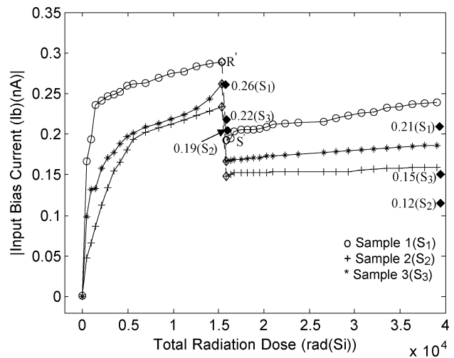
Fig. 8. Variation of I_b of AD549JH, as a function of total irradiation dose.
