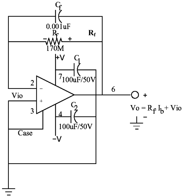
Fig. 1. Circuit schematic used to measure nascent characteristics of ULIBC linear devices.
